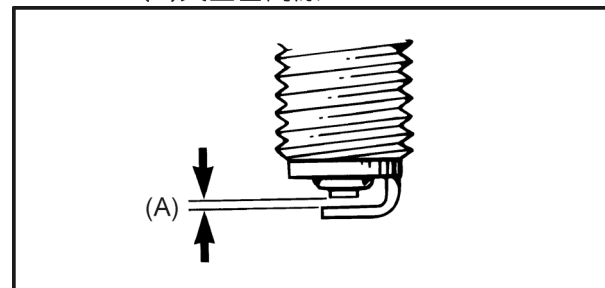
(A) 火星塞間隙0.6~0.7mm
